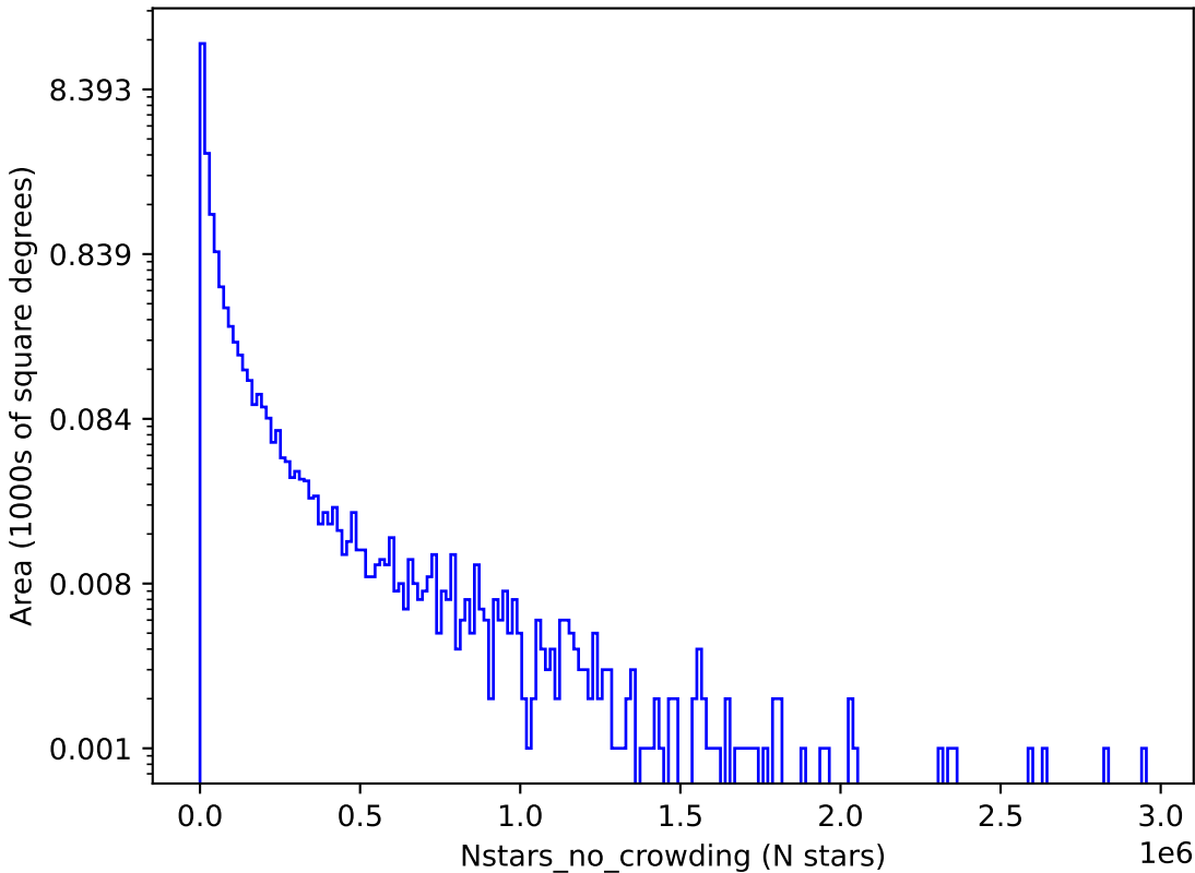
smc_lmc_v3.3_10yrs u: Nstars_no_crowding
