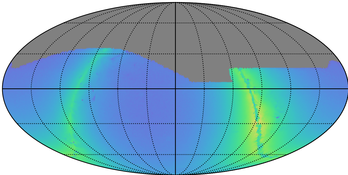
smc_lmc_v3.3_10yrs r: Nstars_no_crowding
