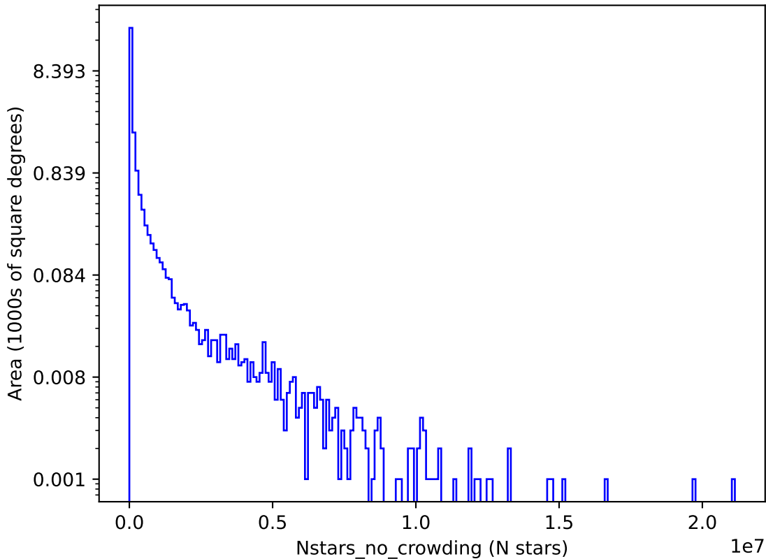
smc_lmc_v3.3_10yrs r: Nstars_no_crowding
