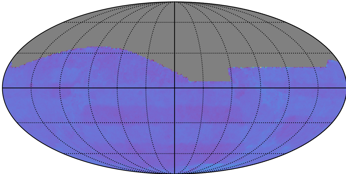
smc_Imc_v3.3_10yrs : Normalized Proper Motion Uncert @ 24.0
