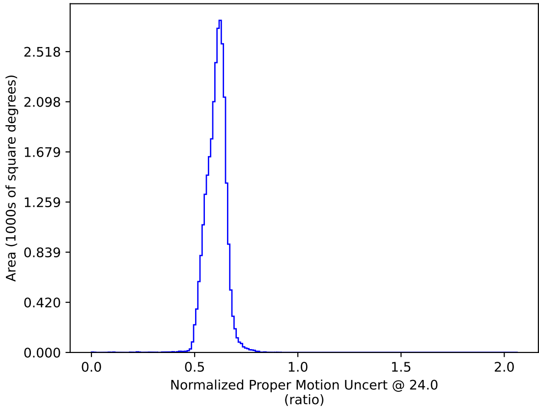
smc_lmc_v3.3_10yrs : Normalized Proper Motion Uncert @ 24.0
