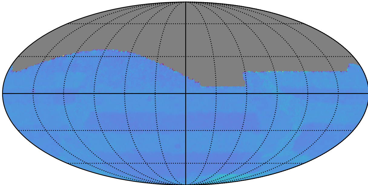
smc_Imc_v3.3_10yrs : Normalized Proper Motion Uncert @ 20.5
