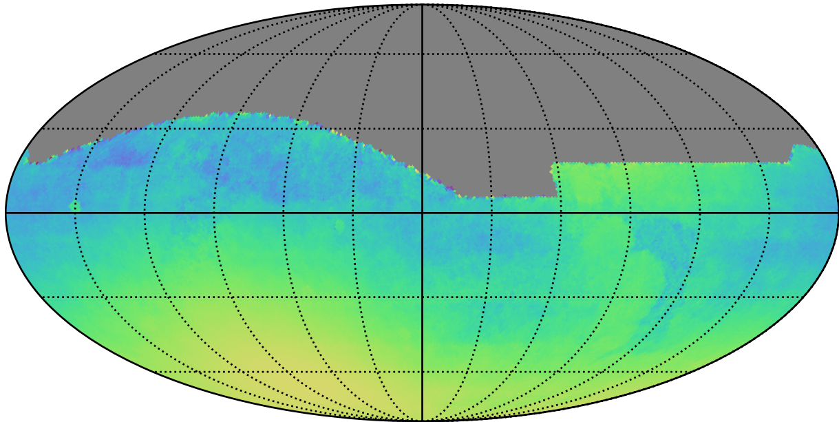
smc_lmc_v3.3_10yrs : Normalized Parallax Uncert @ 24.0
