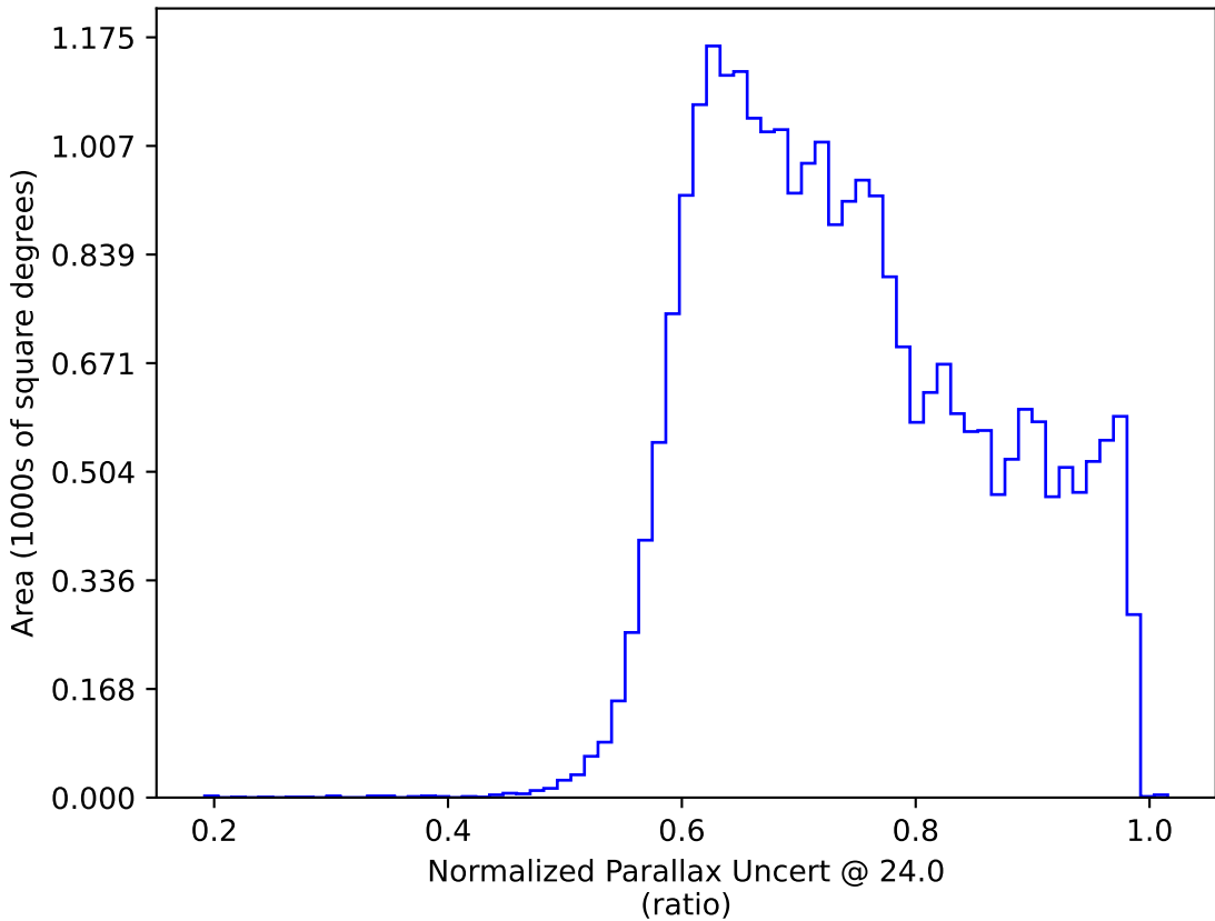
smc_lmc_v3.3_10yrs : Normalized Parallax Uncert @ 24.0
