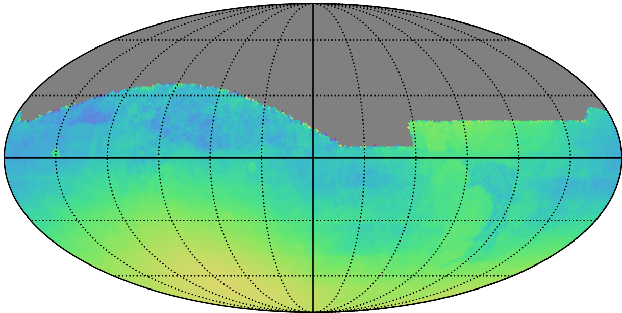
smc_lmc_v3.3_10yrs : Normalized Parallax Uncert @ 22.4
