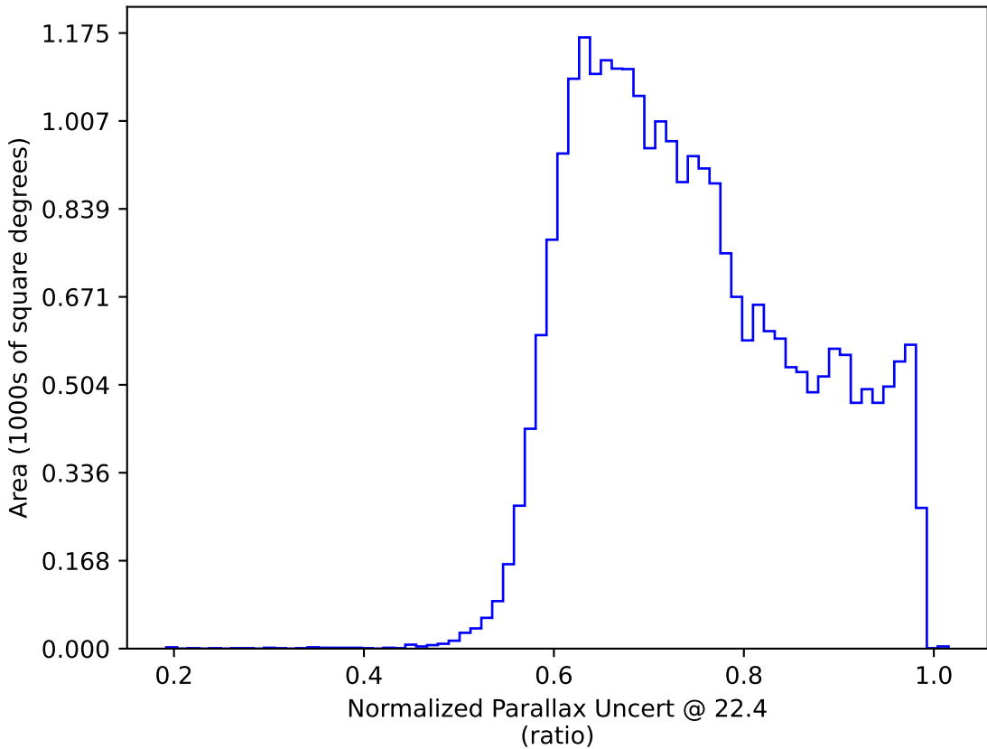
smc_lmc_v3.3_10yrs : Normalized Parallax Uncert @ 22.4
