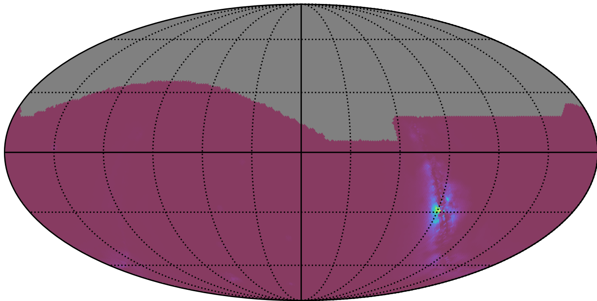
smc_lmc_v3.3_10yrs : NlcPoints
