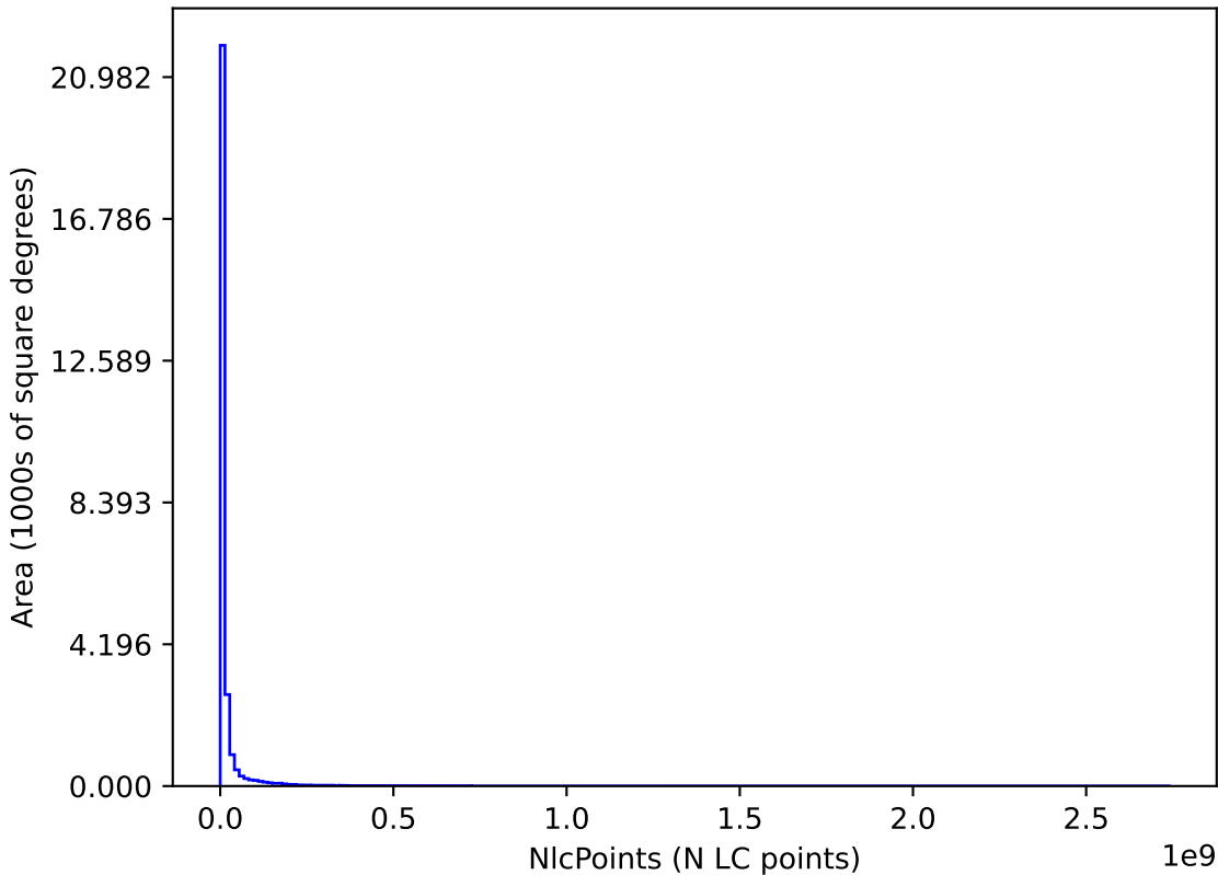
smc_lmc_v3.3_10yrs : NlcPoints
