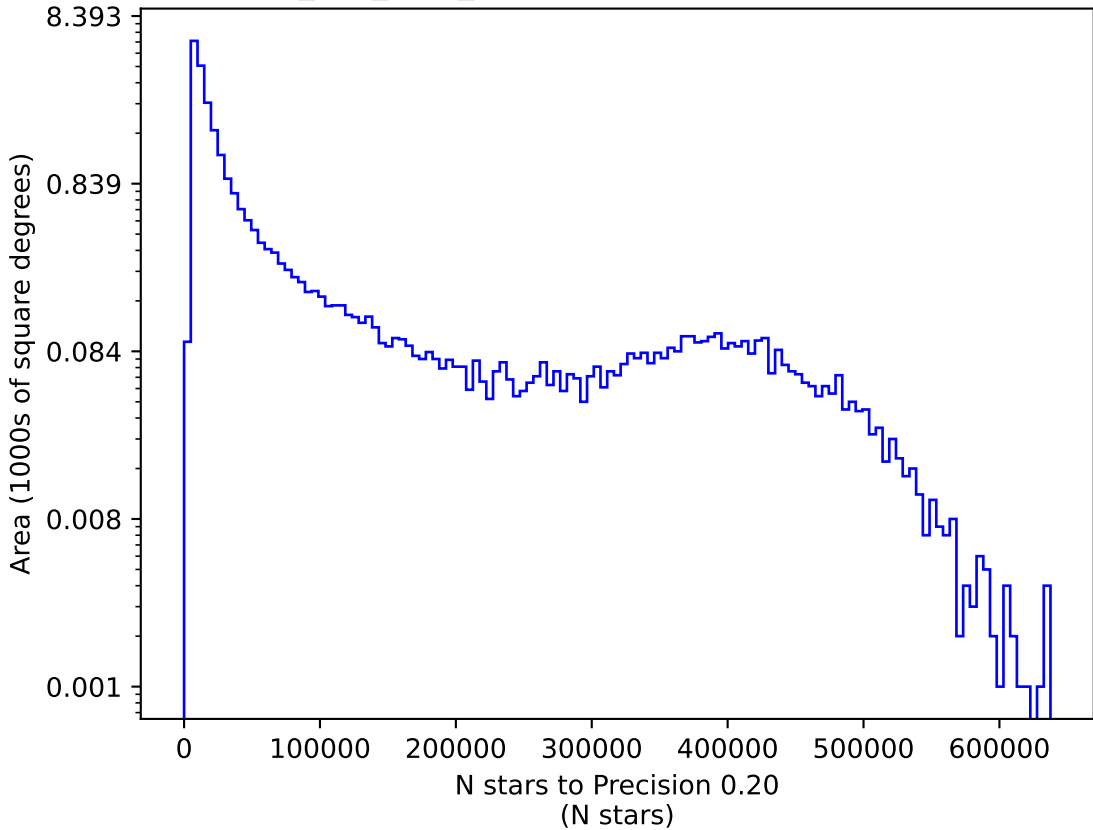
smc_lmc_v3.3_10yrs z: N stars to Precision 0.20
