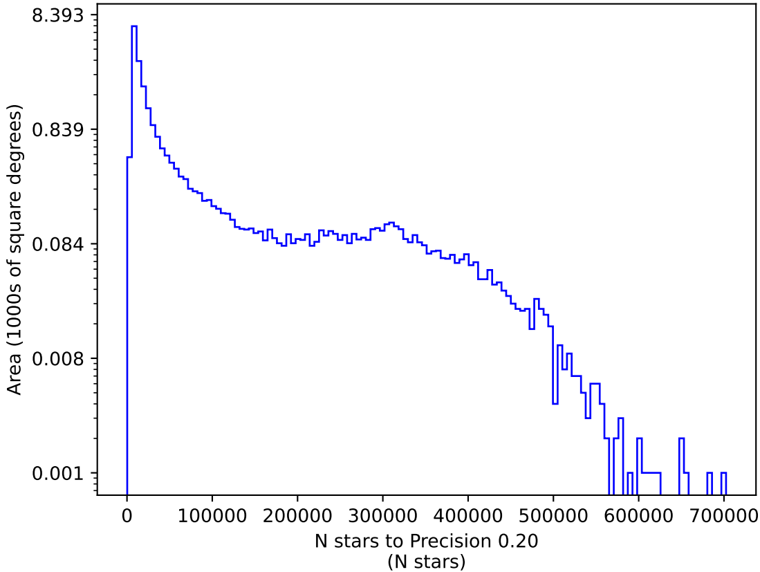
smc_lmc_v3.3_10yrs y: N stars to Precision 0.20
