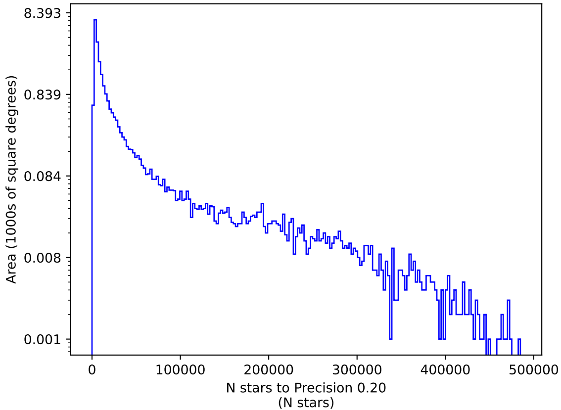
smc_lmc_v3.3_10yrs u: N stars to Precision 0.20
