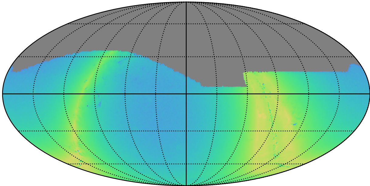
smc_lmc_v3.3_10yrs r: N stars to Precision 0.20
