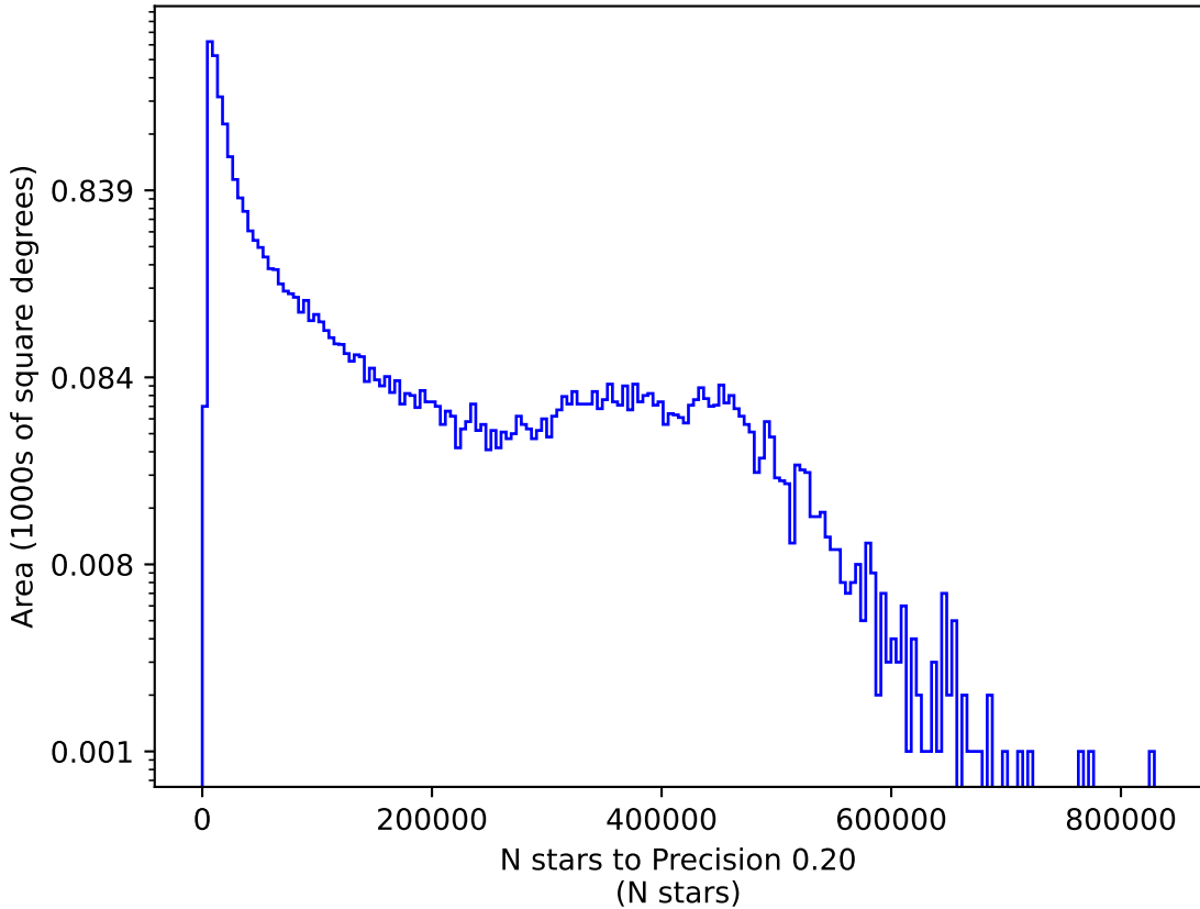
smc_lmc_v3.3_10yrs r: N stars to Precision 0.20
