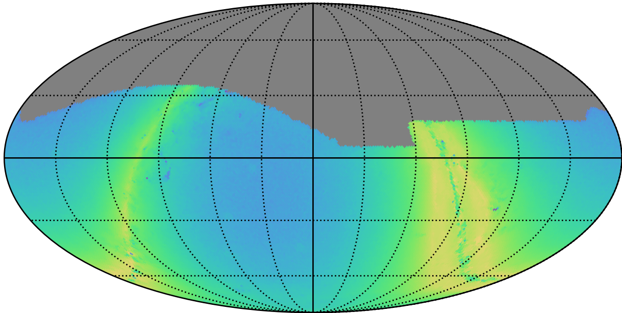
smc_lmc_v3.3_10yrs g: N stars to Precision 0.20
