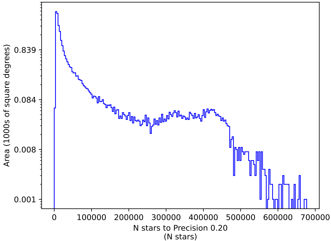
smc_lmc_v3.3_10yrs g: N stars to Precision 0.20
