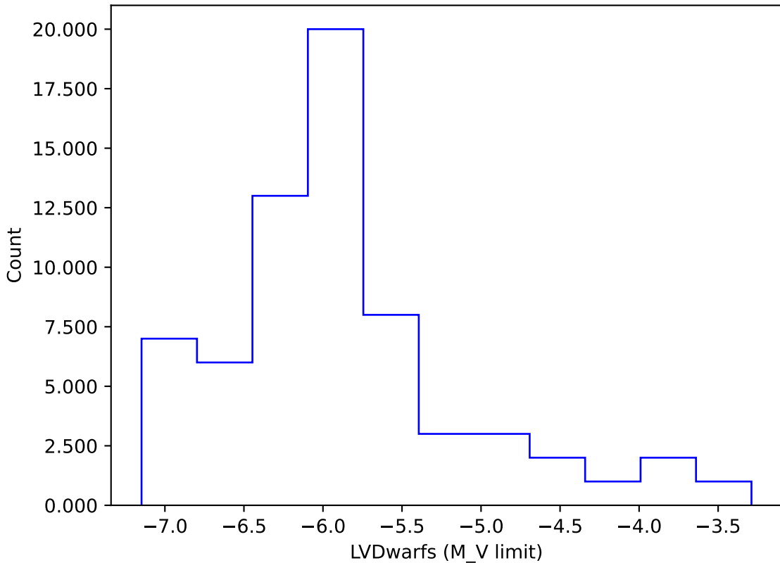
smc_lmc_v3.3_10yrs gi: LVDwarfs
