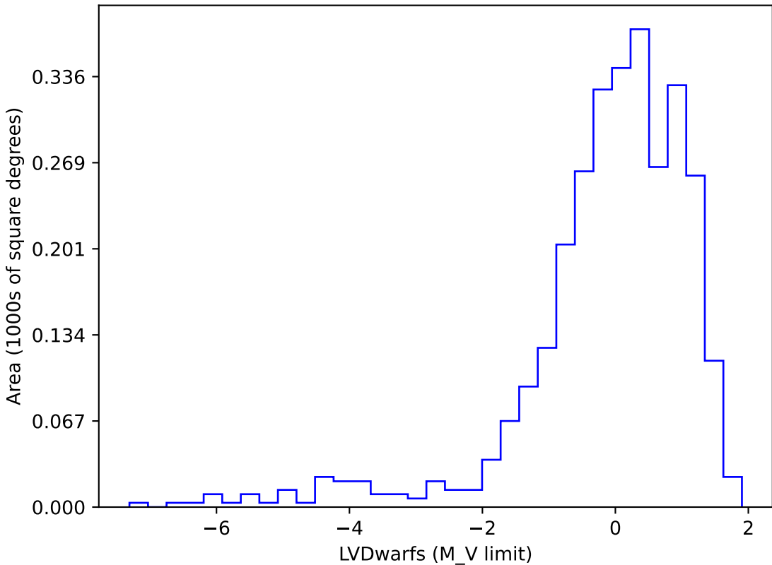
smc_lmc_v3.3_10yrs gi SCP: LVDwarfs
