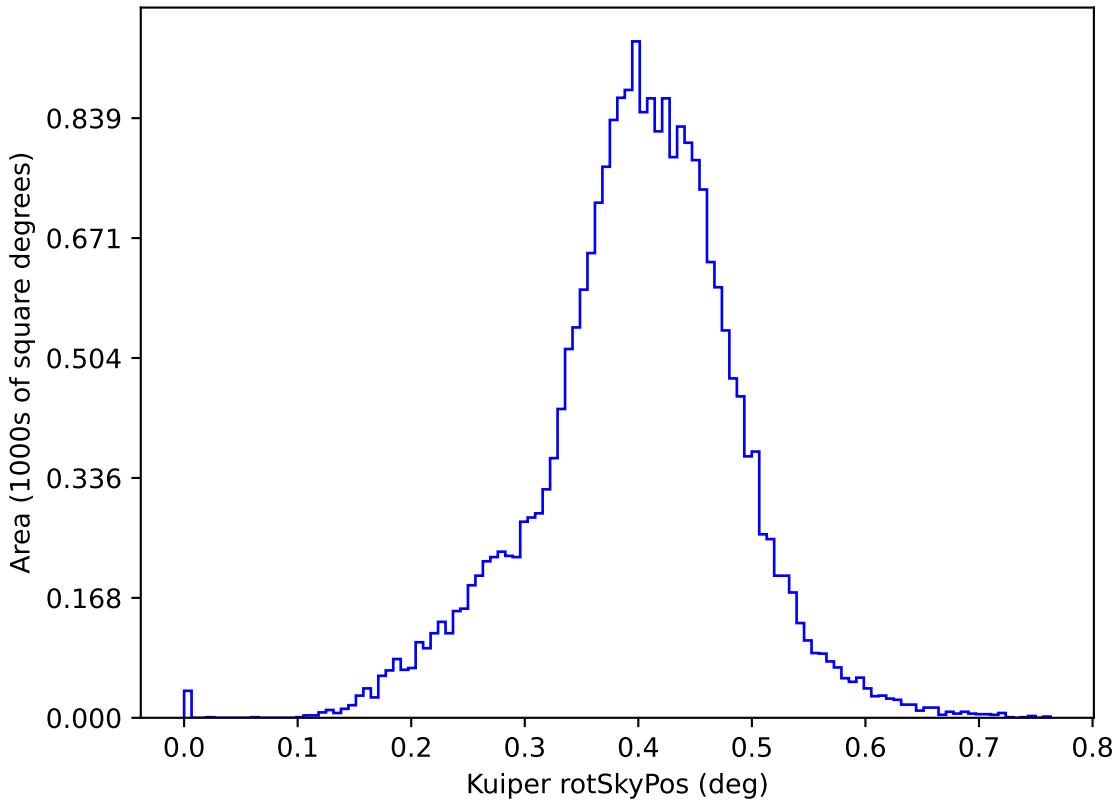
smc_lmc_v3.3_10yrs y: Kuiper rotSkyPos
