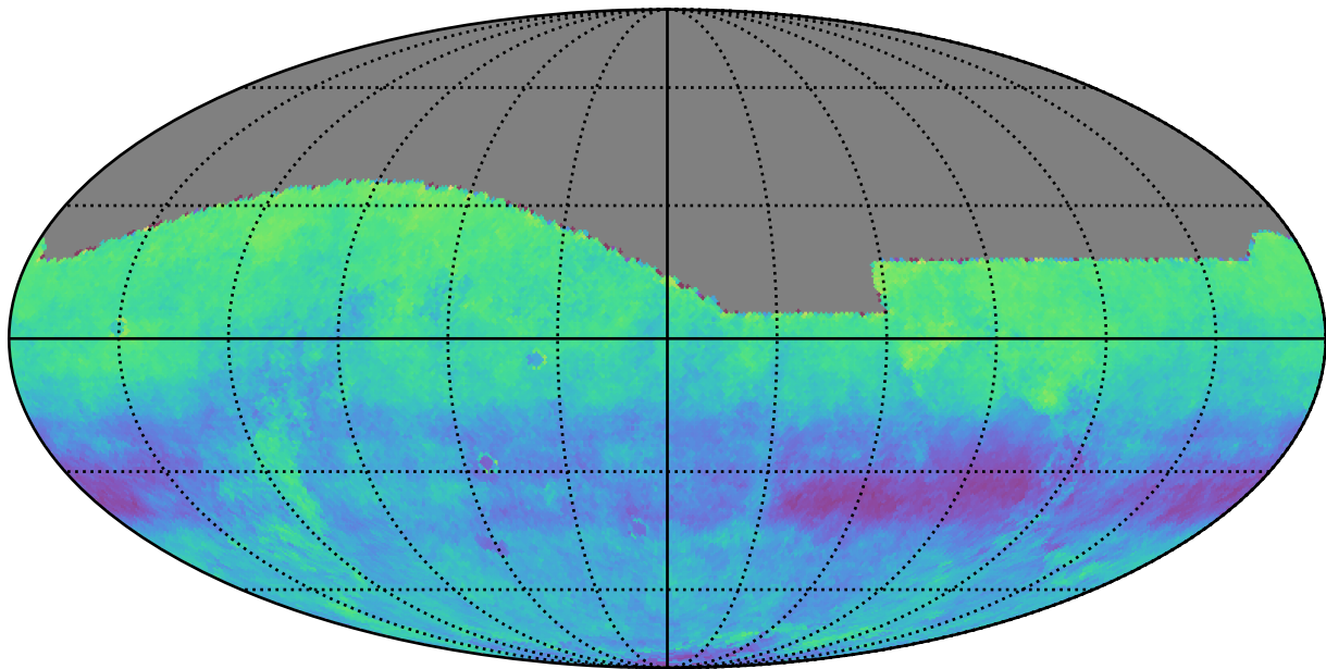
smc_lmc_v3.3_10yrs r: Kuiper rotSkyPos
