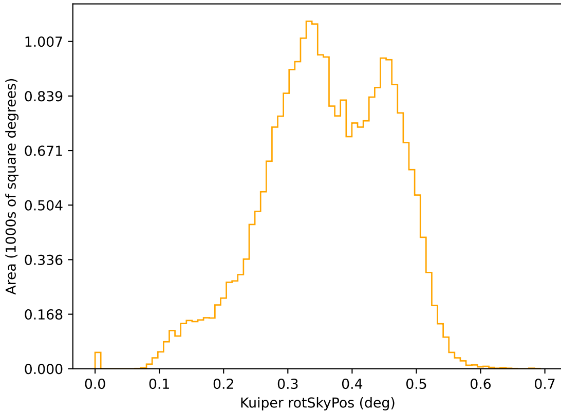
smc_lmc_v3.3_10yrs r: Kuiper rotSkyPos
