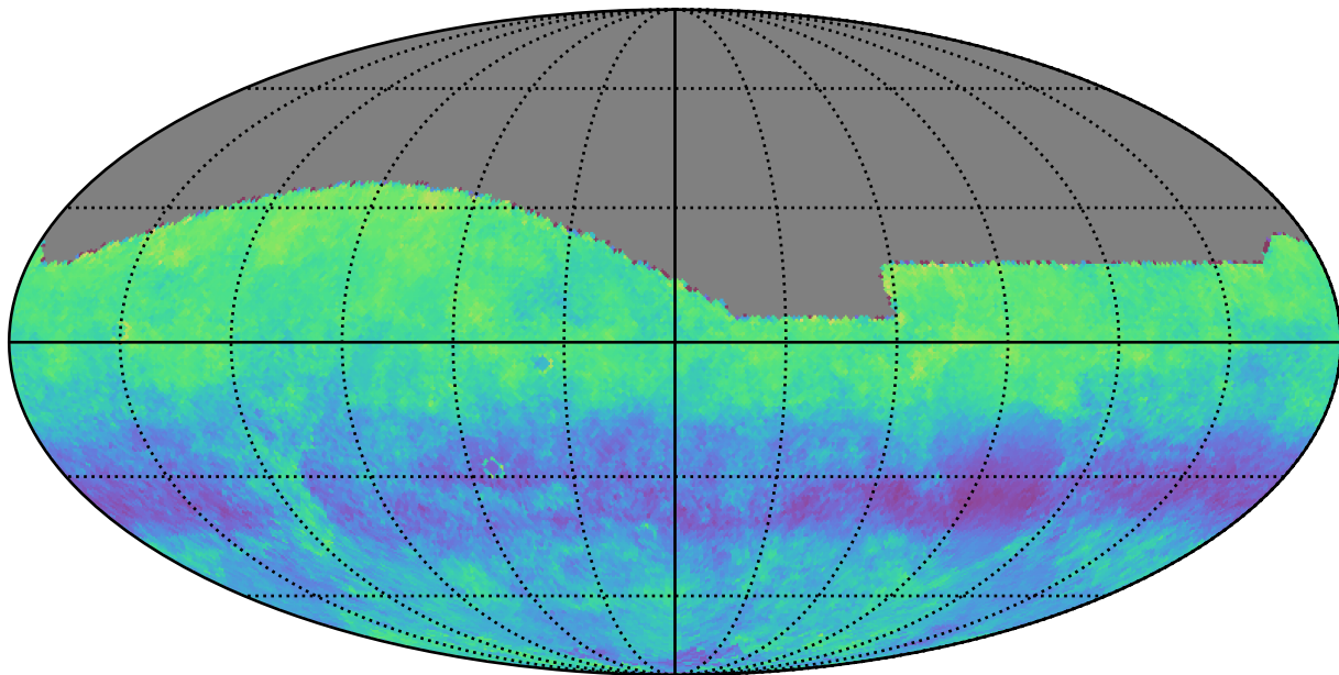
smc_lmc_v3.3_10yrs g: Kuiper rotSkyPos
