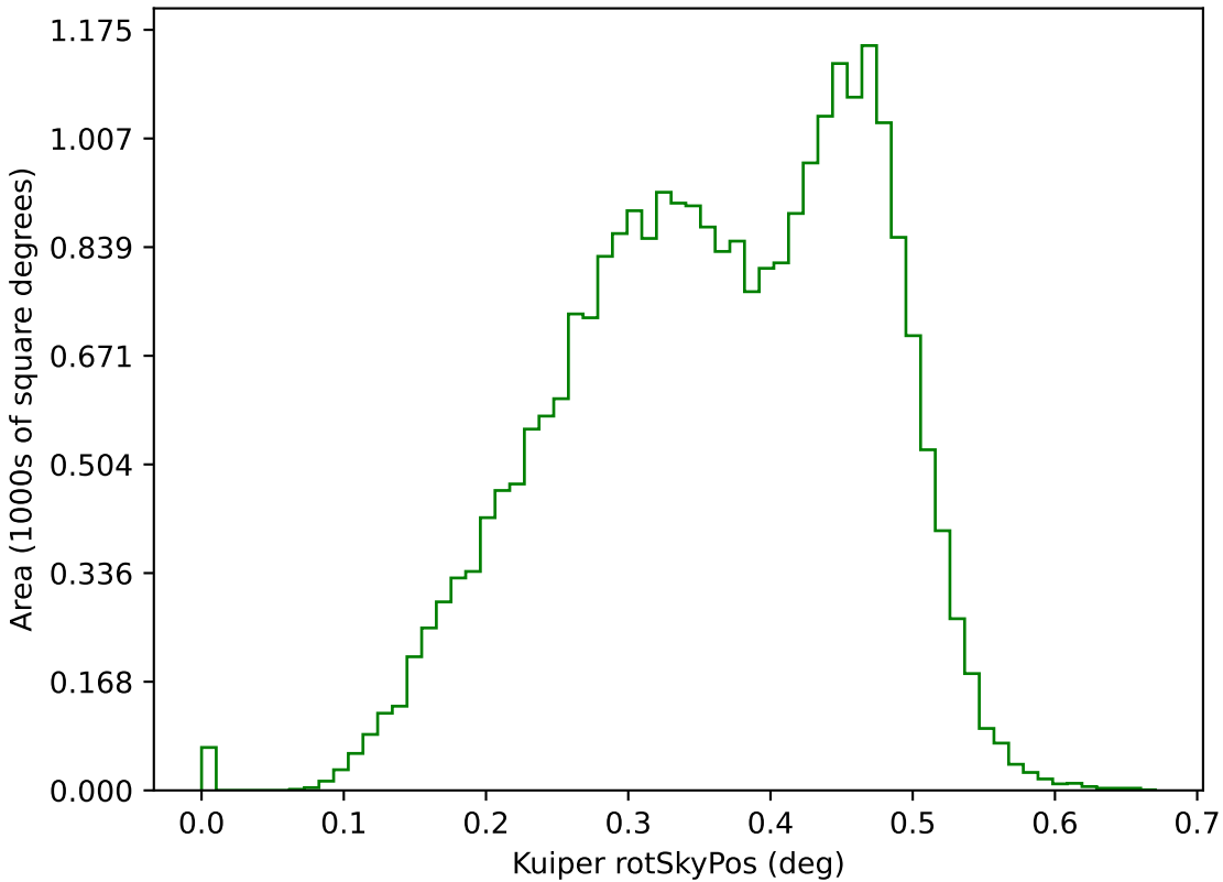
smc_lmc_v3.3_10yrs g: Kuiper rotSkyPos
