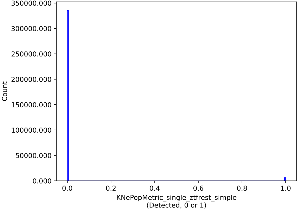
smc_Imc_v3.3_10yrs single model: KNePopMetric_single_ztfrest_simple
