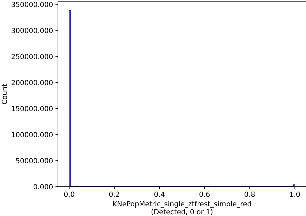
smc_lmc_v3.3_10yrs single model: KNePopMetric_single_ztfrest_simple_red
