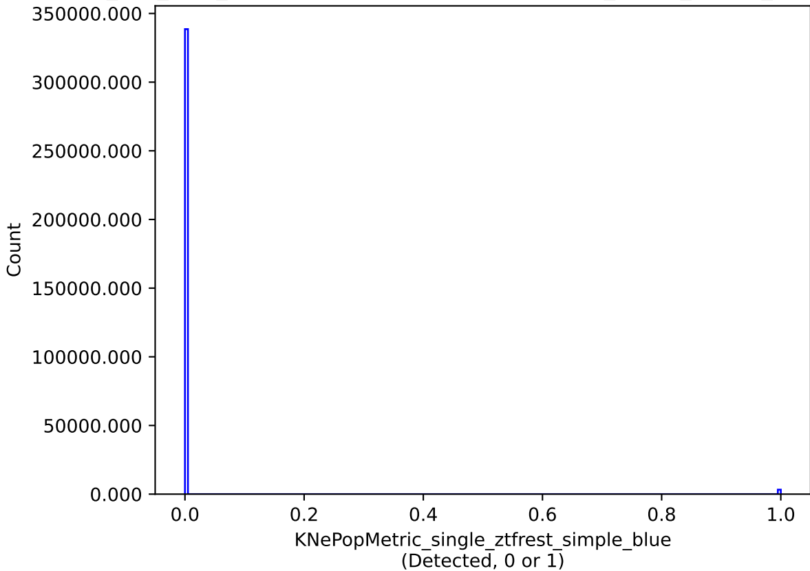
smc_Imc_v3.3_10yrs single model: KNePopMetric_single_ztfrest_simple_blue
