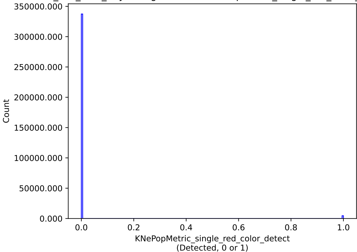
smc_lmc_v3.3_10yrs single model: KNePopMetric_single_red_color_detect
