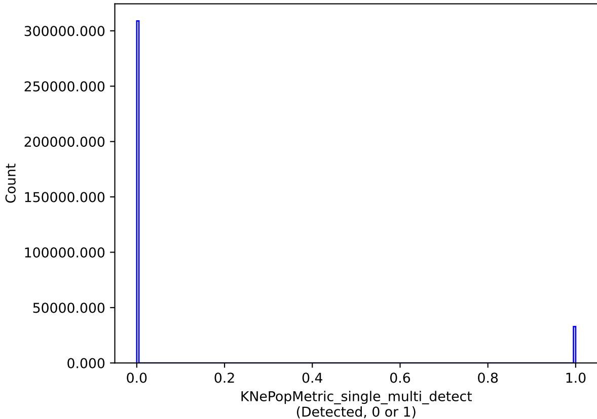
smc_Imc_v3.3_10yrs single model: KNePopMetric_single_multi_detect
