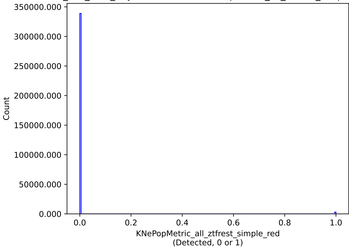
smc_Imc_v3.3_10yrs all models: KNePopMetric_all_ztfrest_simple_red
