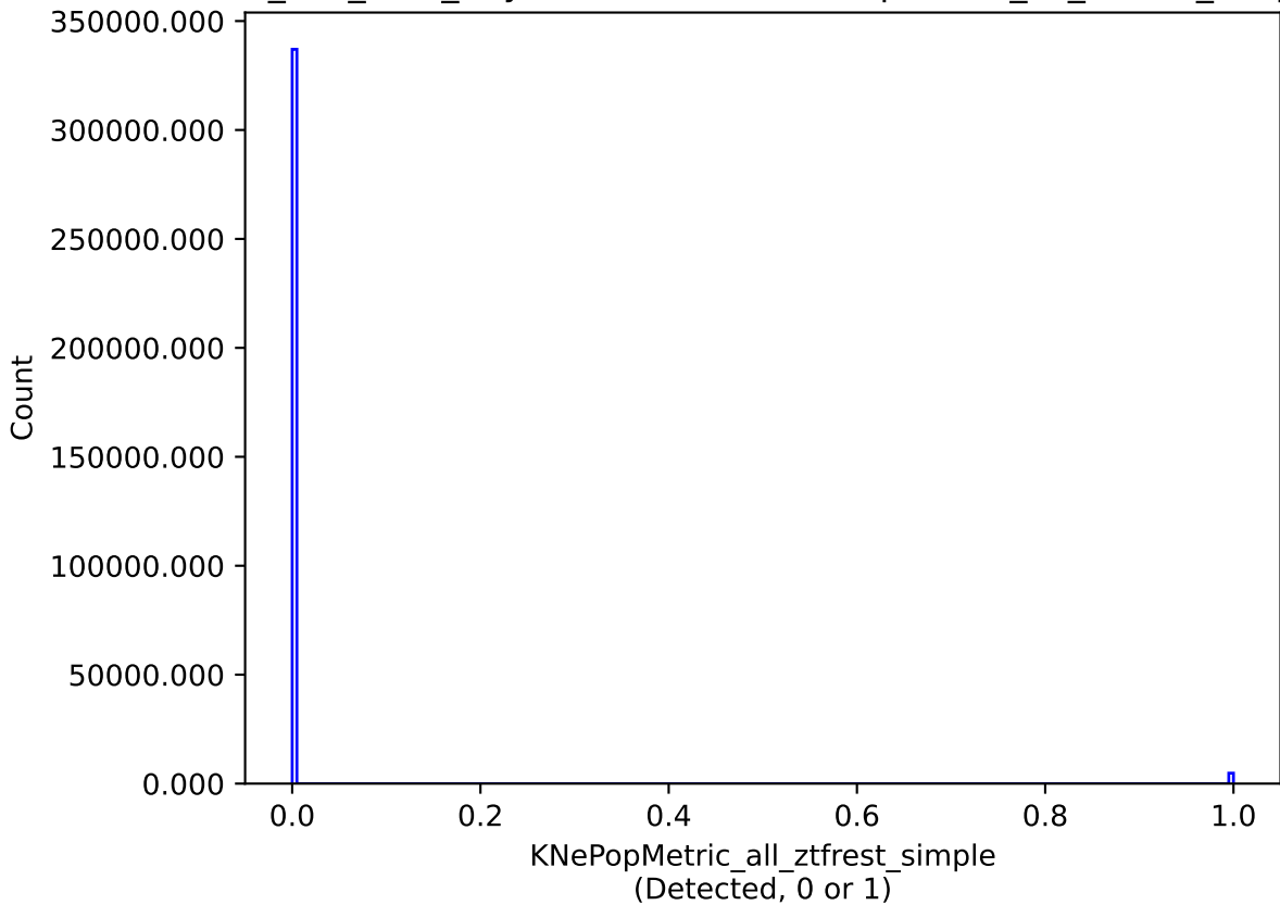
smc_lmc_v3.3_10yrs all models: KNePopMetric_all_ztfrest_simple
