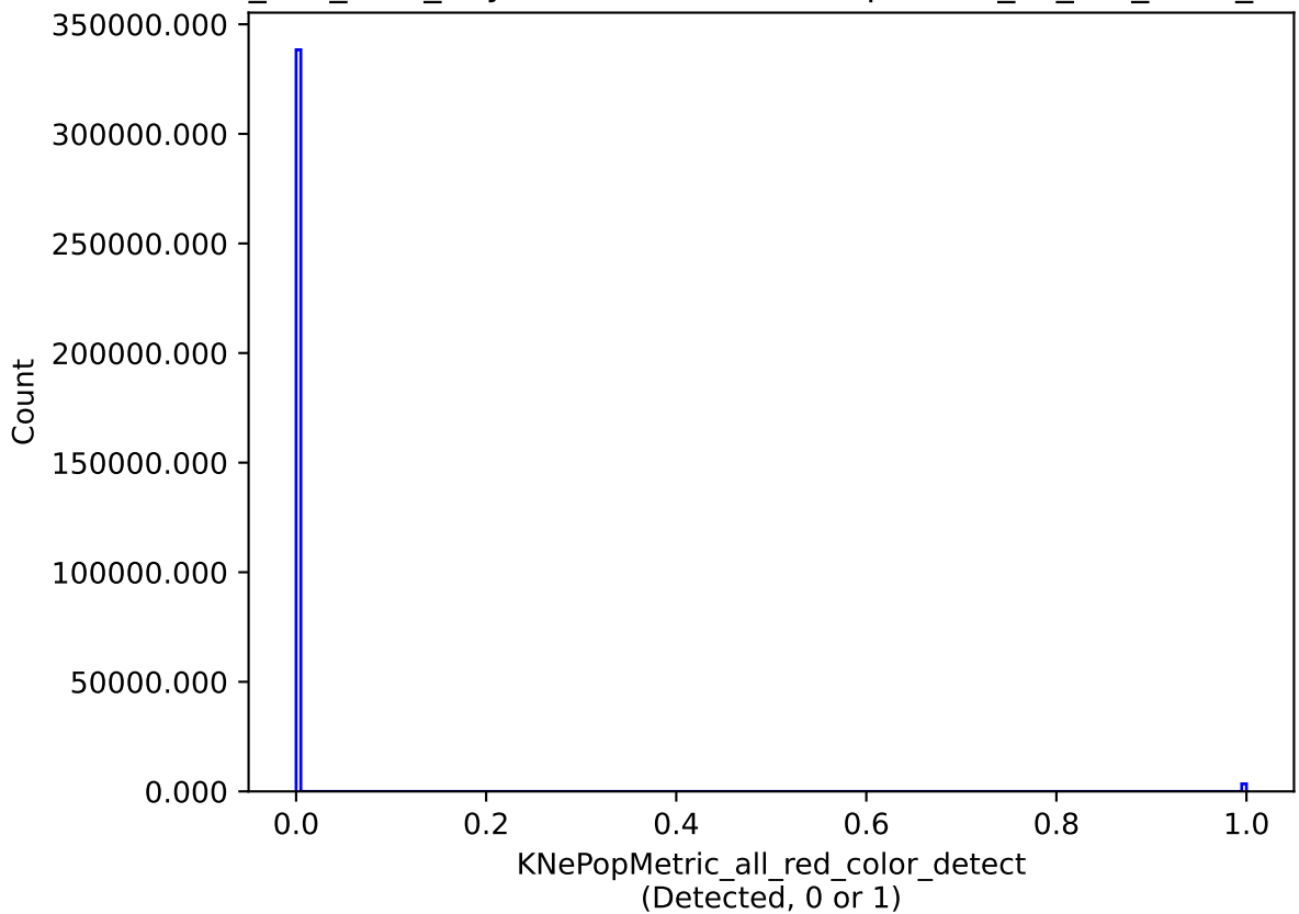
smc_lmc_v3.3_10yrs all models: KNePopMetric_all_red_color_detect
