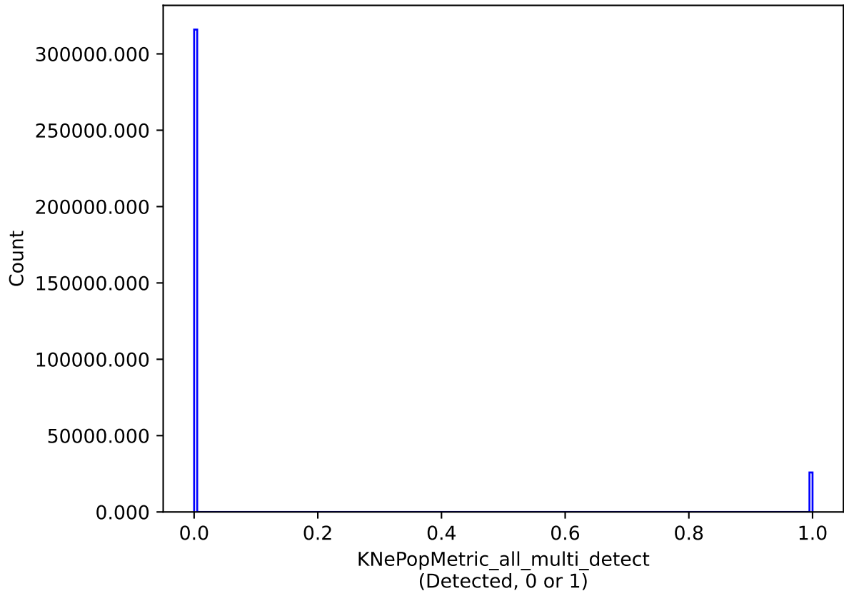
smc_lmc_v3.3_10yrs all models: KNePopMetric_all_multi_detect
