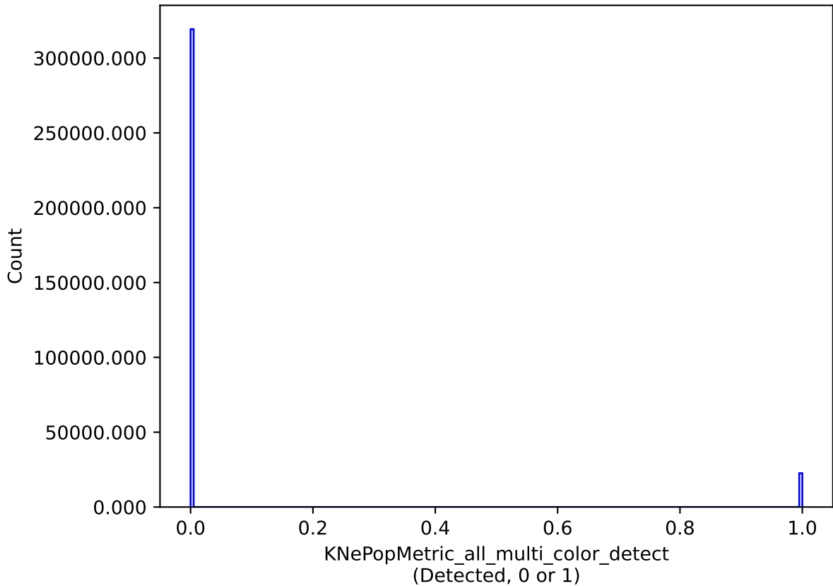
smc_lmc_v3.3_10yrs all models: KNePopMetric_all_multi_color_detect
