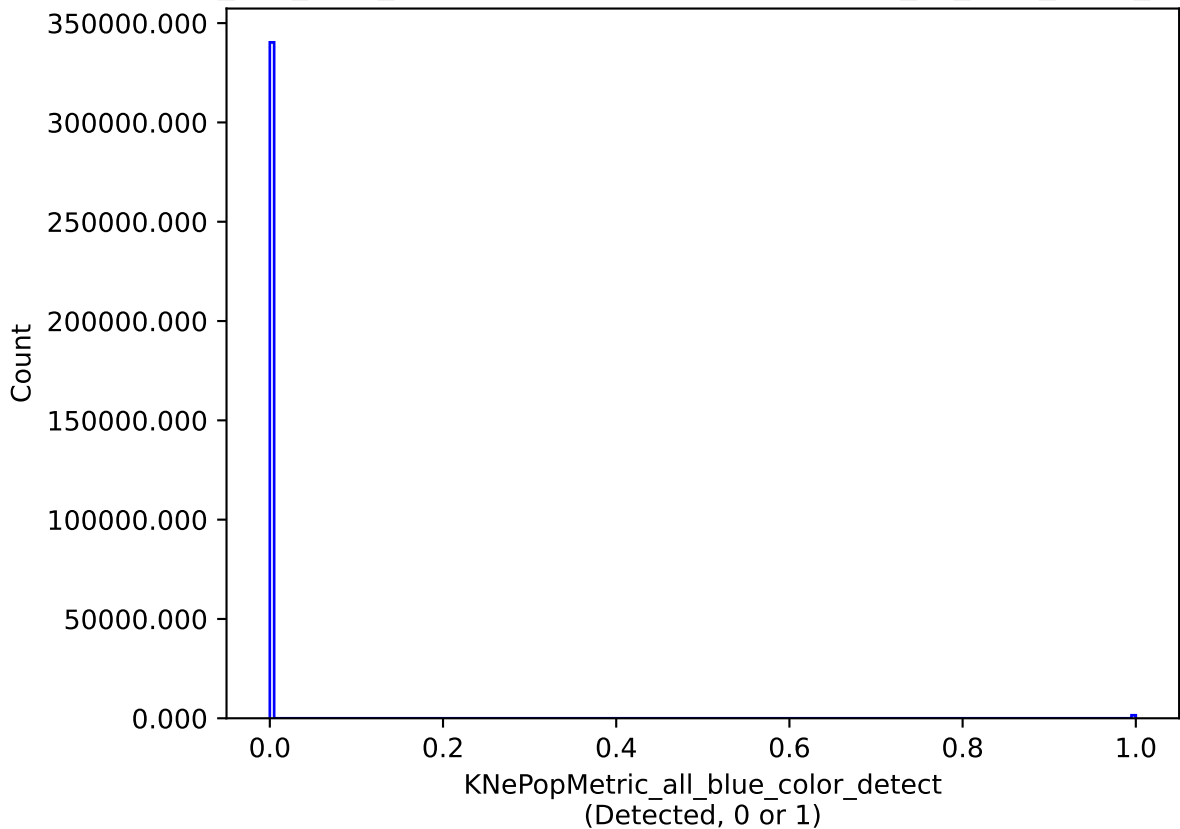
smc_lmc_v3.3_10yrs all models: KNePopMetric_all_blue_color_detect
