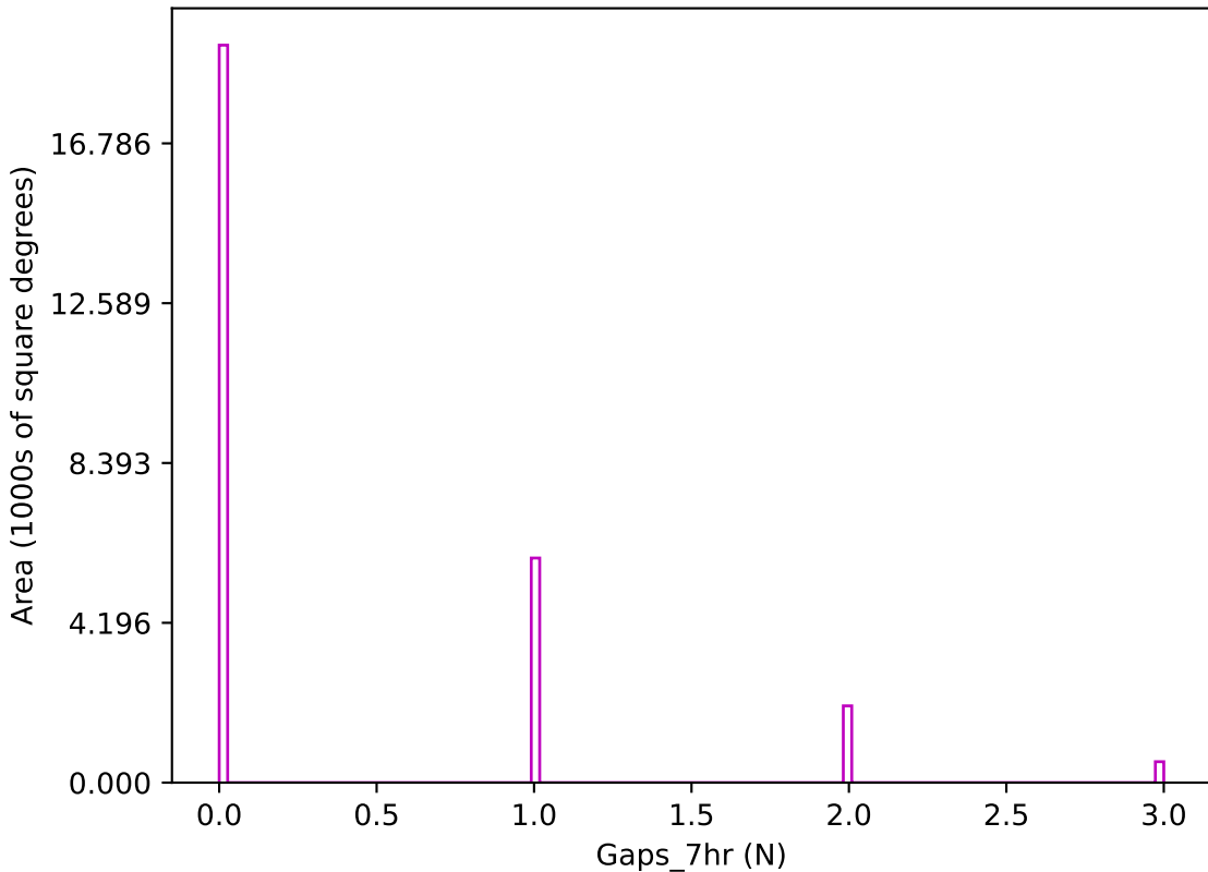
smc_lmc_v3.3_10yrs z band: Gaps_7hr
