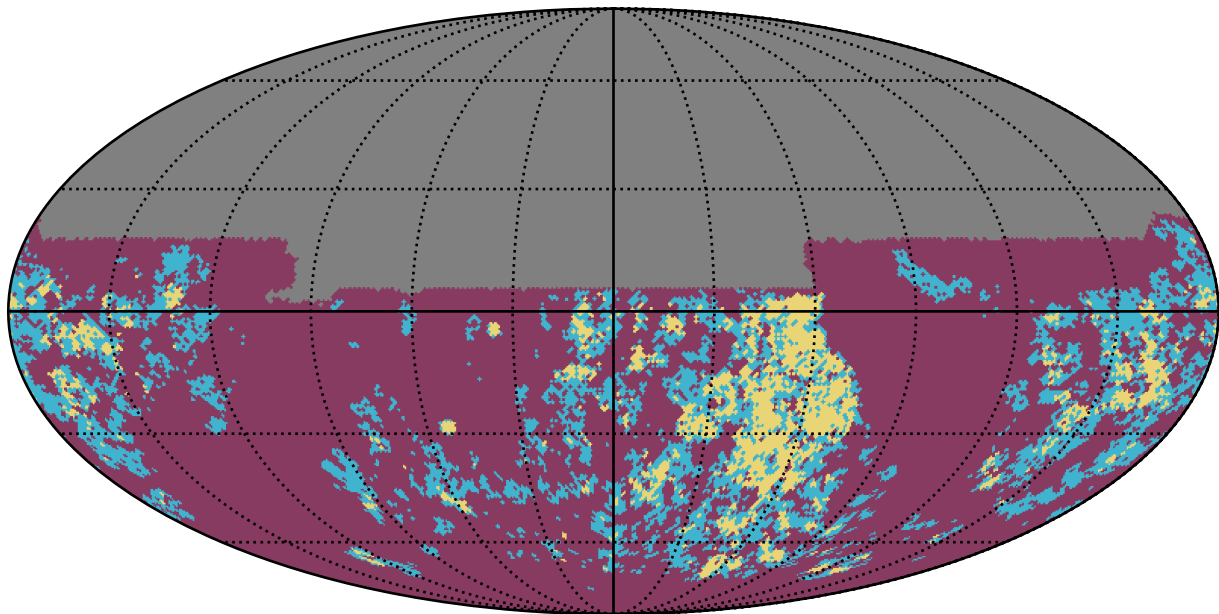
smc_lmc_v3.3_10yrs y band: Gaps_7hr
