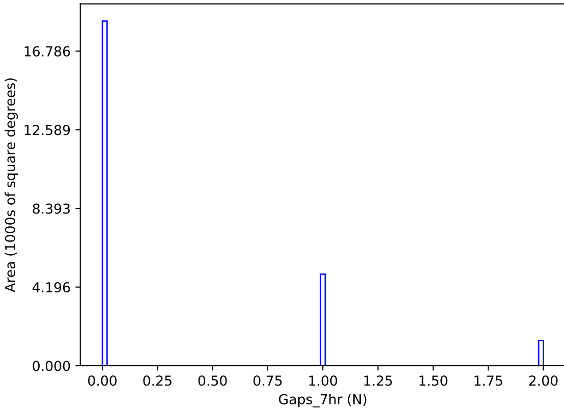
smc_lmc_v3.3_10yrs y band: Gaps_7hr
