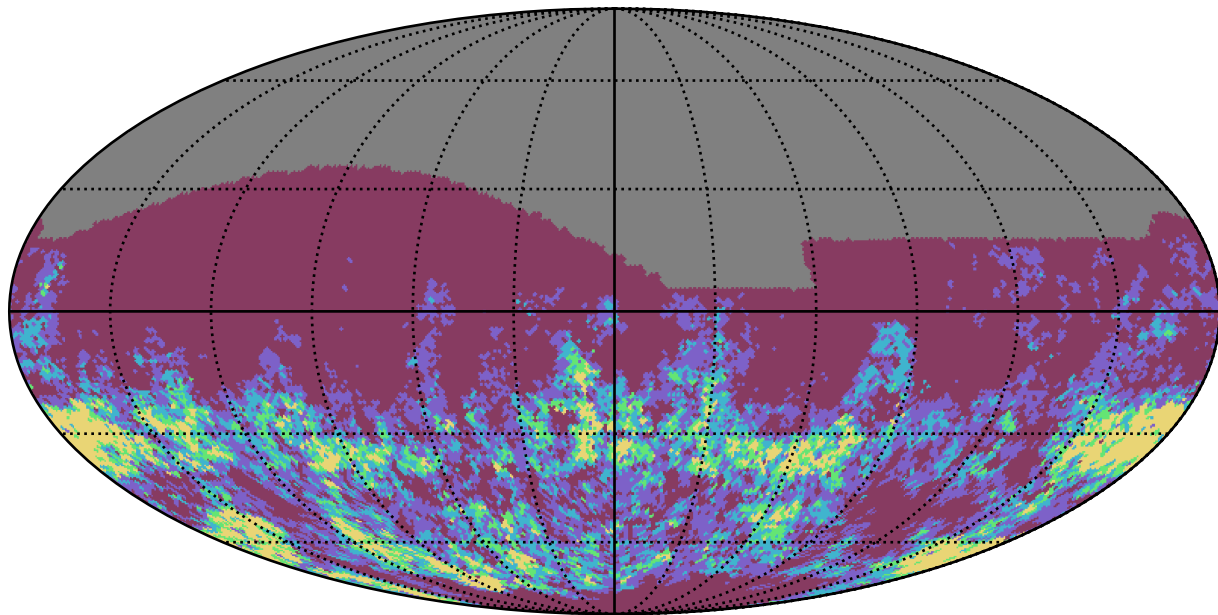
smc_lmc_v3.3_10yrs r band: Gaps_7hr
