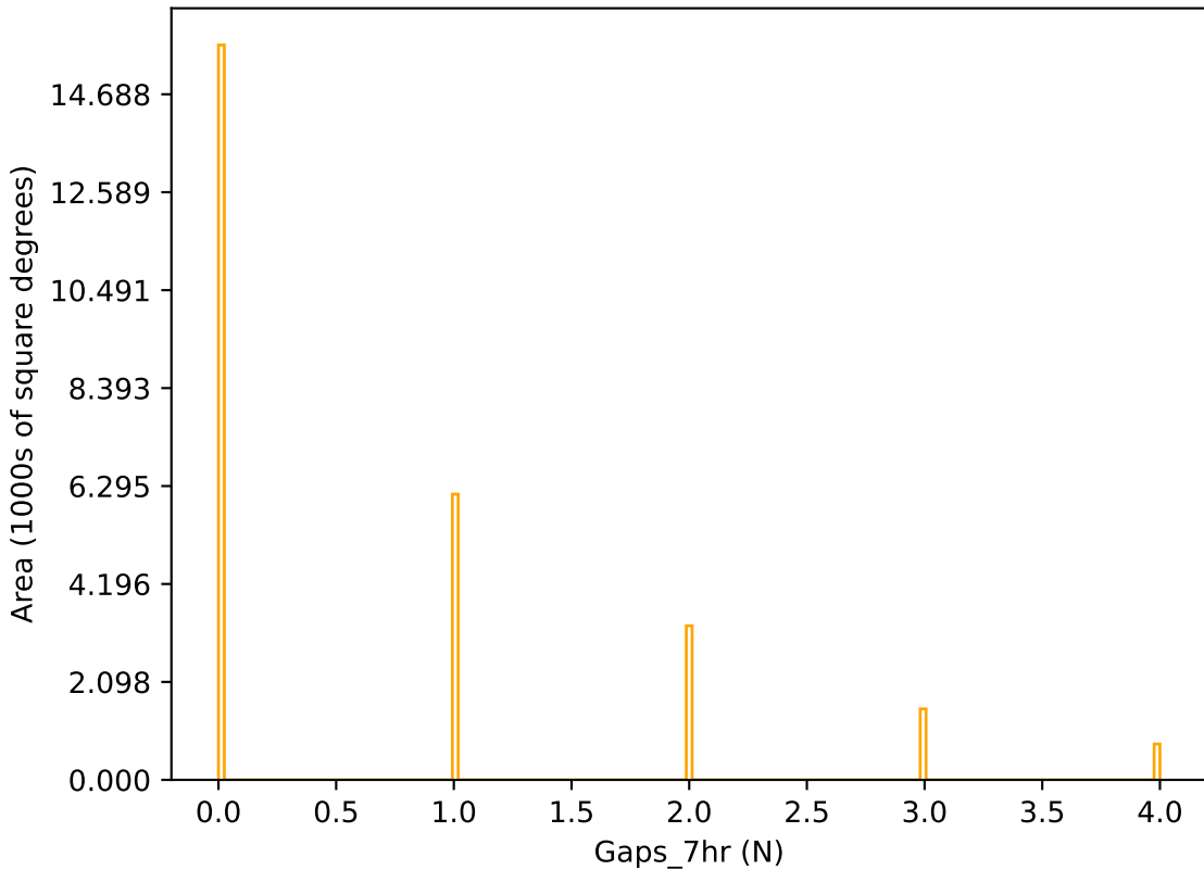
smc_lmc_v3.3_10yrs r band: Gaps_7hr
