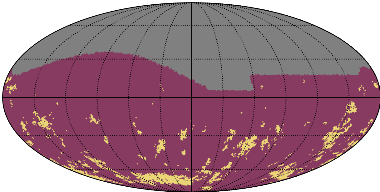
smc_lmc_v3.3_10yrs g band: Gaps_7hr
