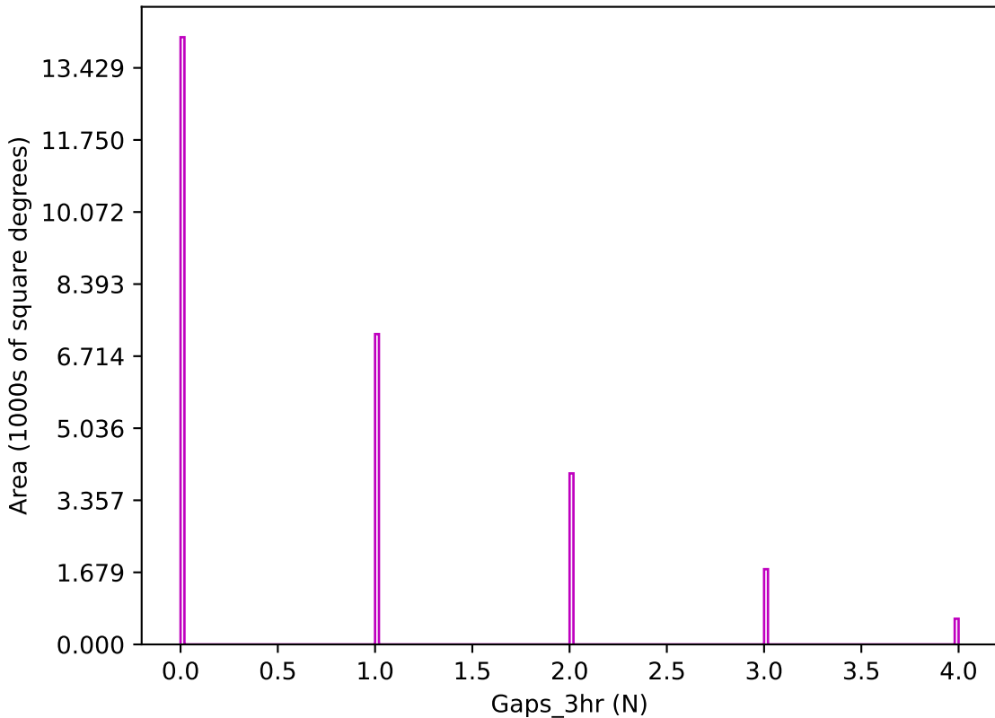
smc_lmc_v3.3_10yrs z band: Gaps_3hr
