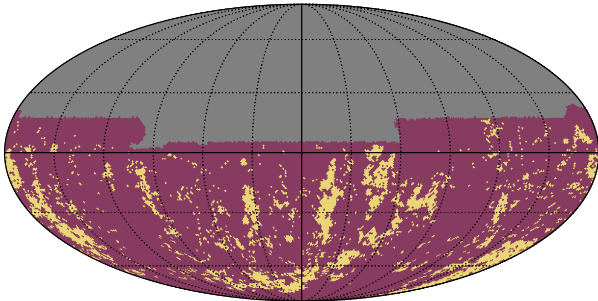
smc_lmc_v3.3_10yrs u band: Gaps_3hr
