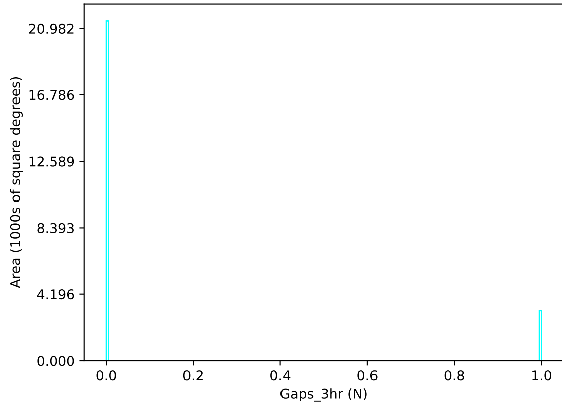
smc_lmc_v3.3_10yrs u band: Gaps_3hr
