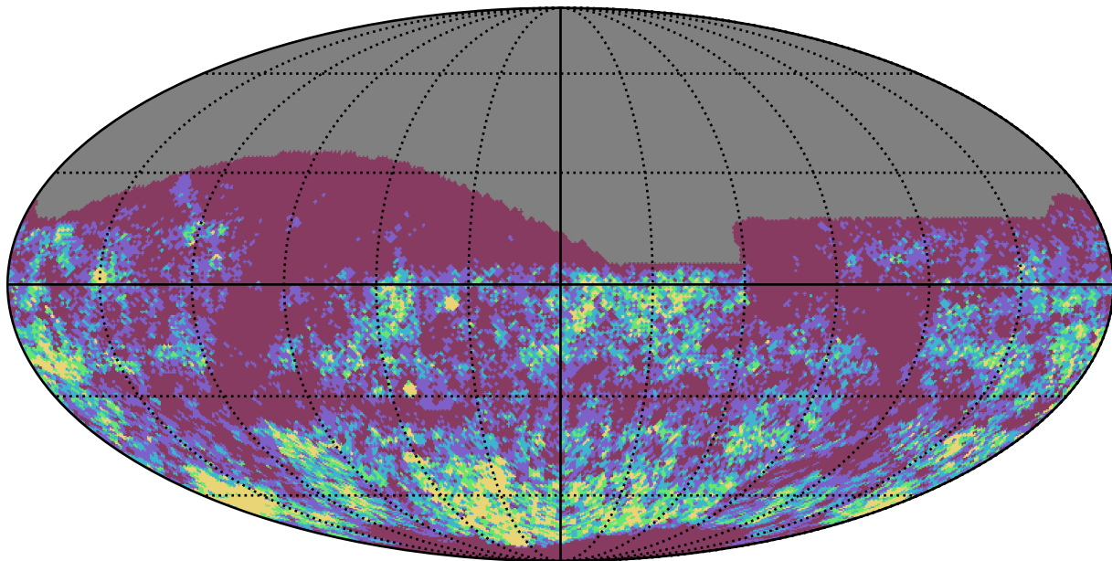
smc_lmc_v3.3_10yrs i band: Gaps_3hr
