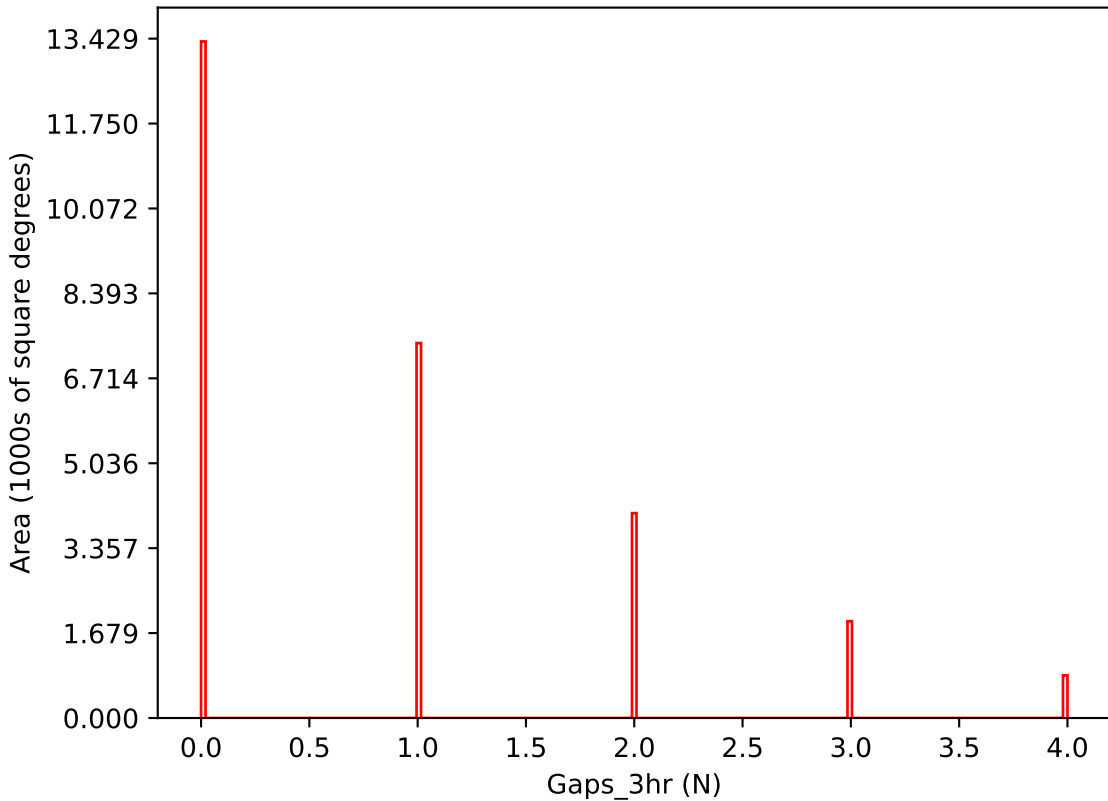
smc_lmc_v3.3_10yrs i band: Gaps_3hr
