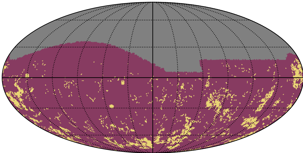
smc_lmc_v3.3_10yrs g band: Gaps_3hr
