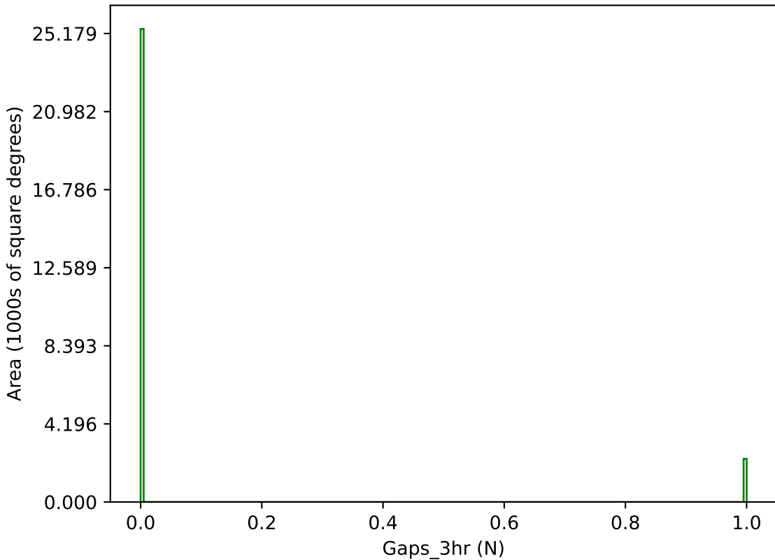
smc_lmc_v3.3_10yrs g band: Gaps_3hr
